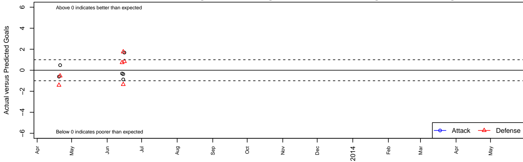
THUSC Cobalt B95 Dots are actual minus expected GF (blue circles) and GA (red triangles). Blue line is smoothed change in attack strength. Red is smoothed change in defense strength.
